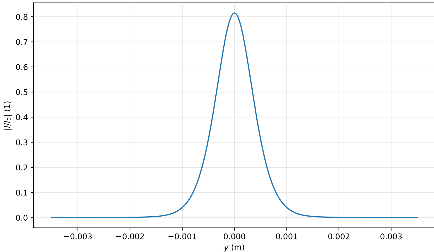
Intensity profile I(x=0, y, z=3.105)/I_0 , P_{in}=0.7P_{cr} , artificial time
